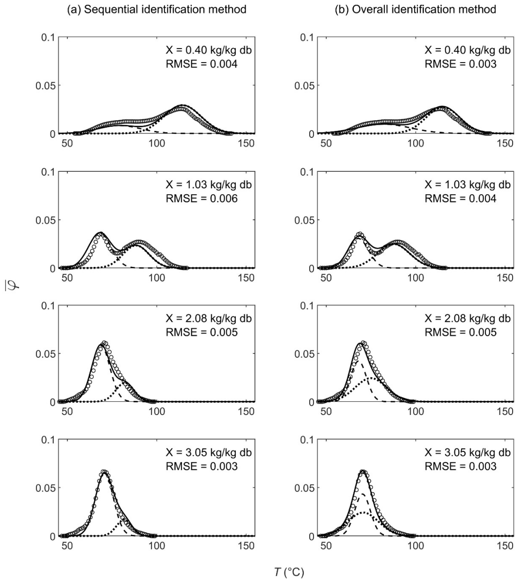
377 378 Figure 4. DSC thermograms of bean starch at different water contents X : experimental (dots) 379 and predicted (solid lines) dimensionless heat flows, predicted G (--) and M (···) endotherms. 380 Predicted data were obtained using the sequential (a) and overall (b) identification method. 381 RMSE were calculated between experimental and predicted dimensionless heat flows for the 382 different water contents. 383
