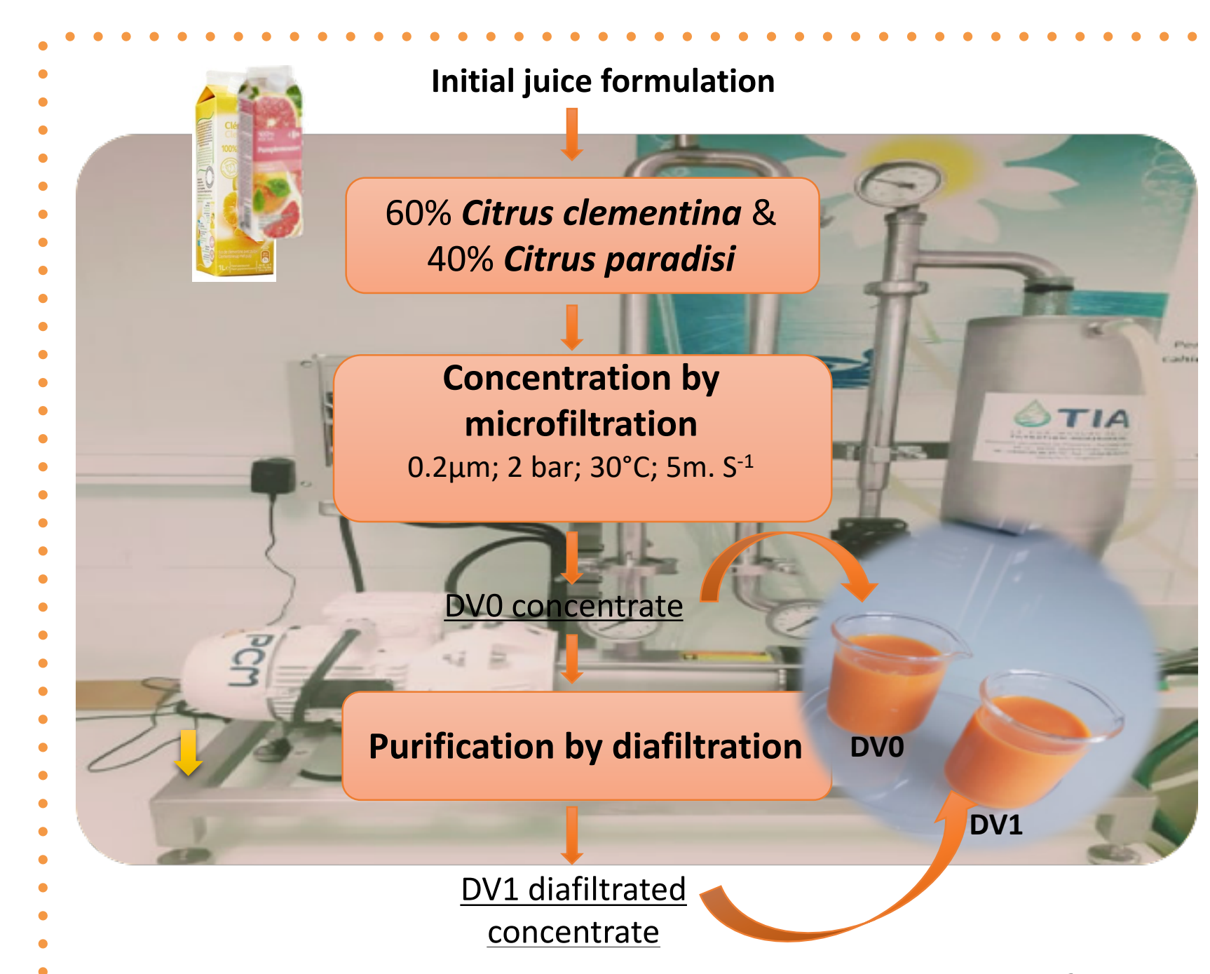
Figure 1. Pilot and Flow diagram for the concentration and purification processes.
