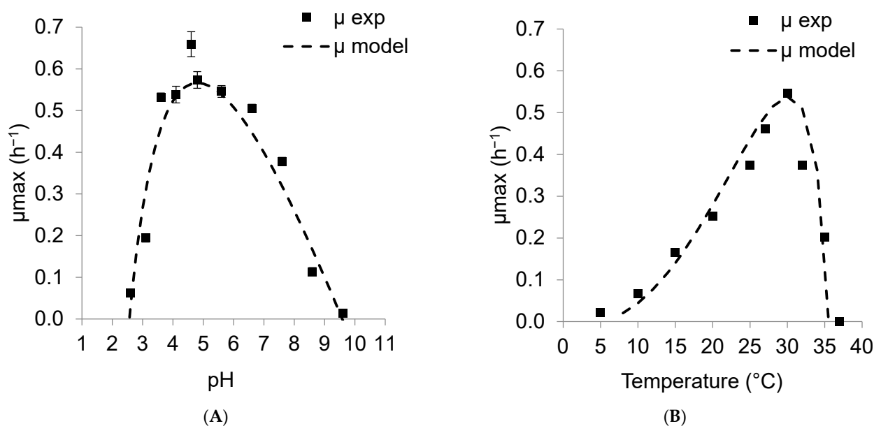
Figure 2. Effect of environmental factors (A) pH and (B) temperature on growth rate of K. unispora . Experimental data (symbols) and predicted data from CTP model (continuous lines).
