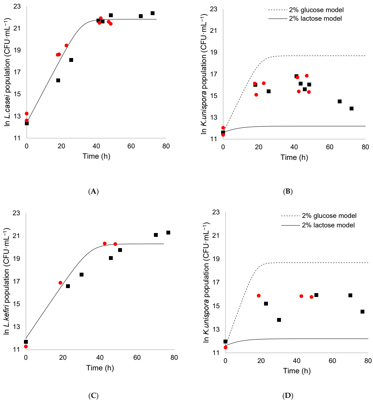
Figure 5. L. casei and K. unispora coculture (A,B), and L. kefirii and K. unispora coculture (C,D) with initial population of each strain of 10^5 CFU·mL -1 in modified MRS (■) and reconstituted mare milk (●). (A) Experimental L. casei population at 25 °C. (B) Experimental population of K. unispora at 25 °C. (C) Experimental L. kefirii population at 30 °C. (D) Experimental population of K. unispora at 30 °C. Lines represent theoretical monoculture growth in lactose (plain line) for LAB and in glucose (dotted lines) and lactose (plain line) for K. unispora .
